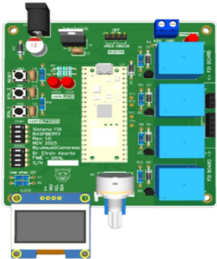
TOP PCB VIEW
