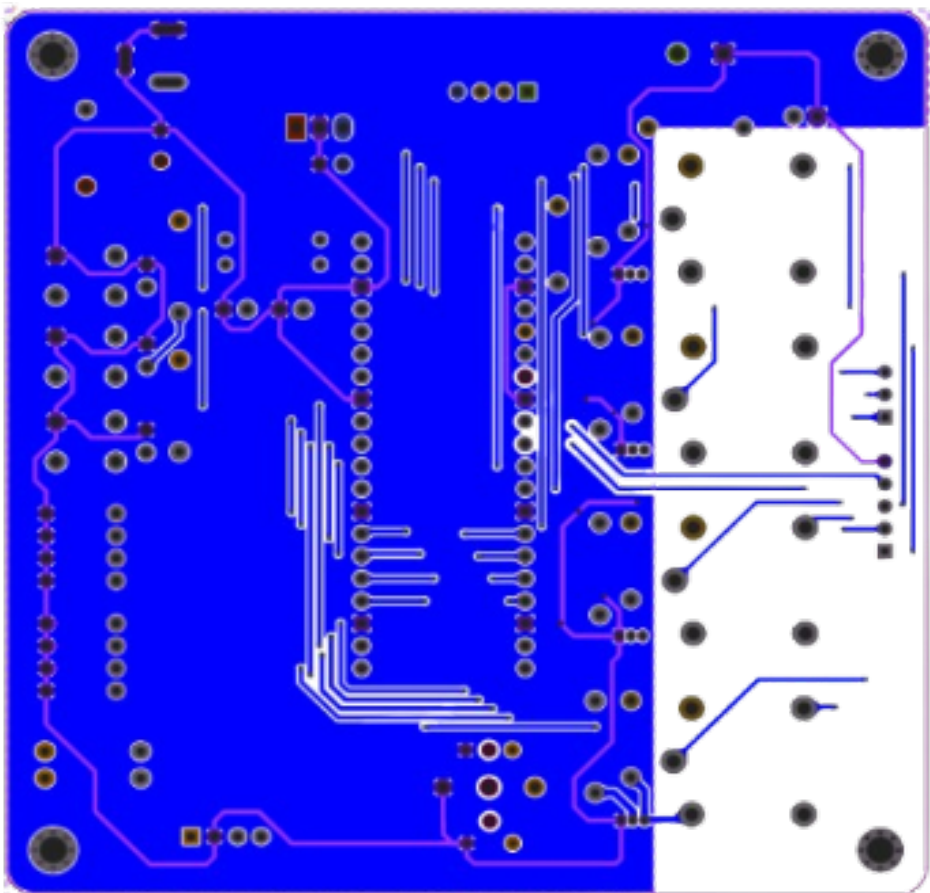
BOTTOM VIEW
