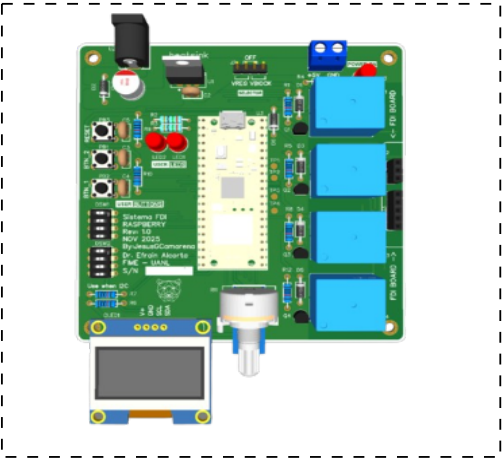
TOP PCB VIEW
